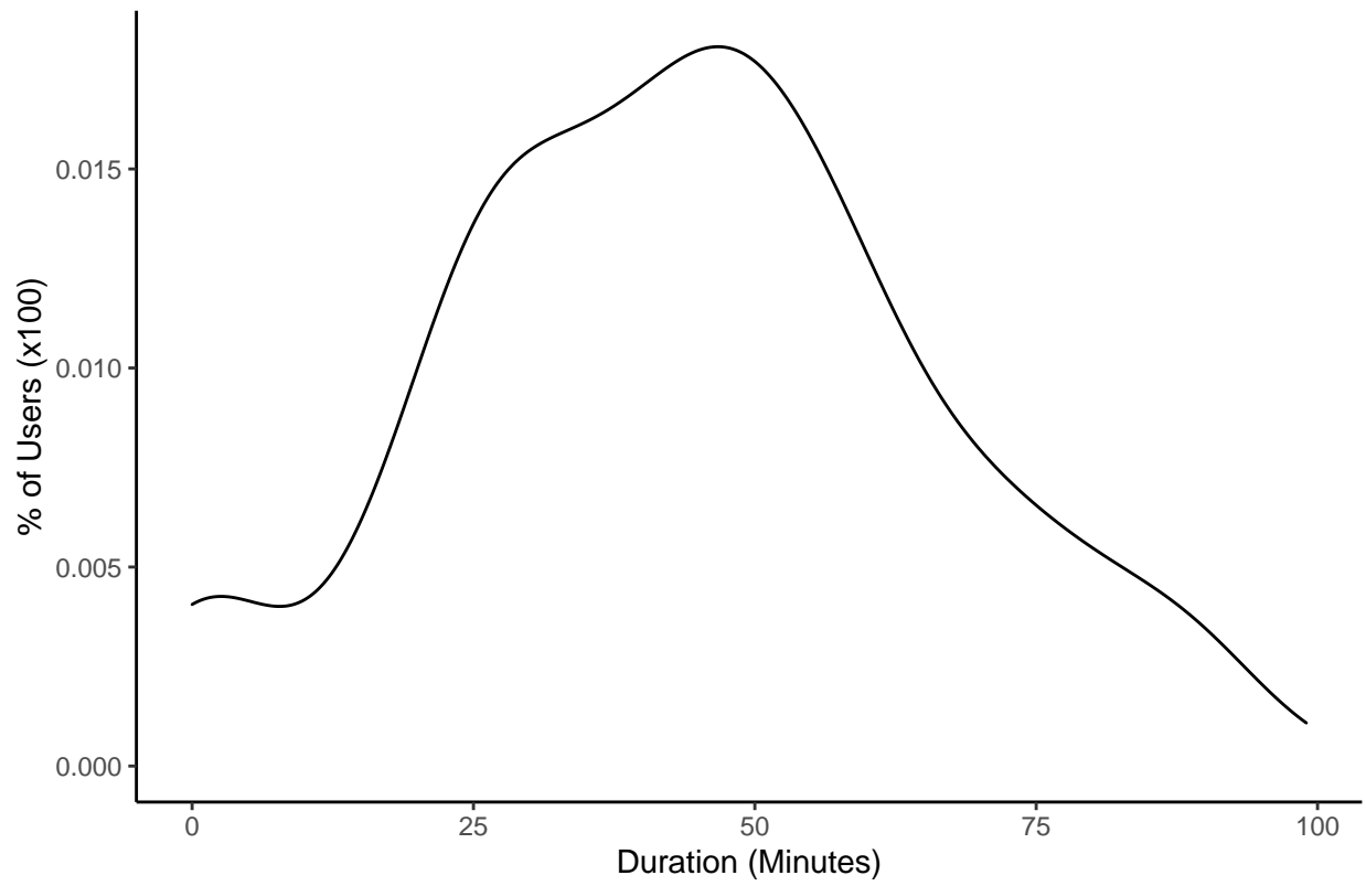
User Average Trip Length (Normal Distribution Detail)
