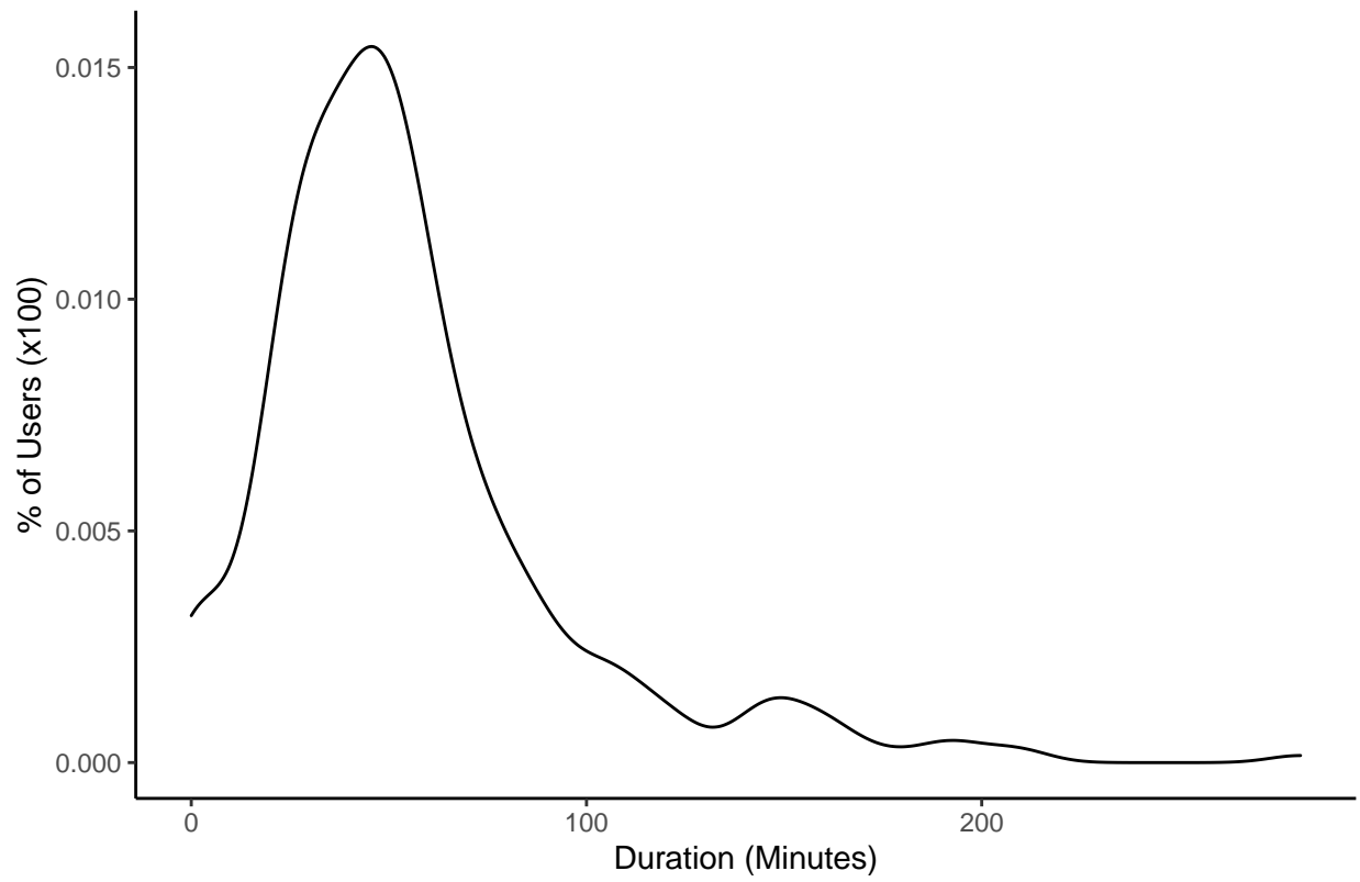
User Average Trip Length Distribution
